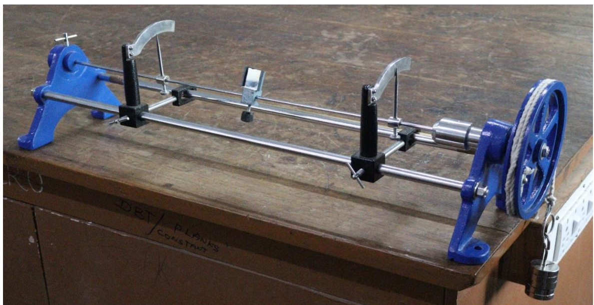
Rigidity Modulus Apparatus
