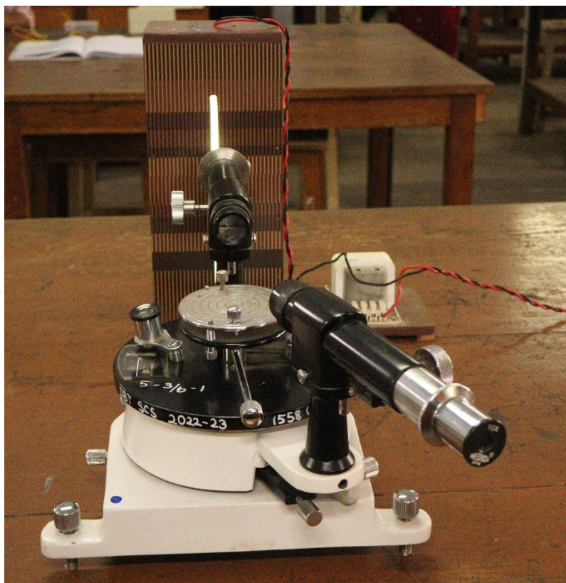
Mercury Vapour lamp and Spectrometer
